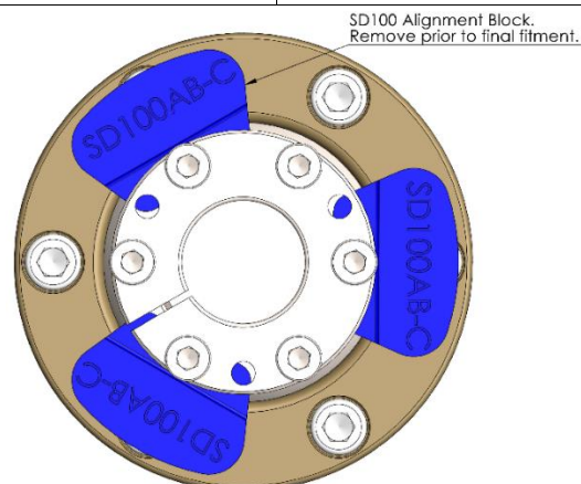
Fig 1. Alignment block
