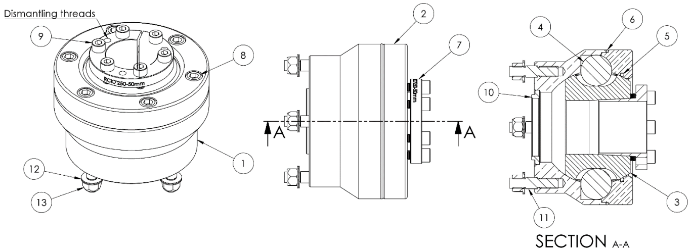
Fig 4. Parts Diagram
