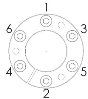
Fig 3. Tightening Sequence
